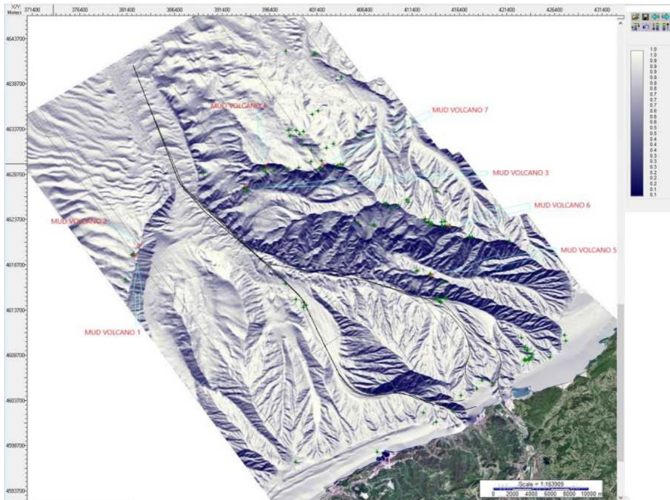
Figure 6-1: Geomorphological map of the offshore area, including the Aol, showing the pipeline route and the location of the closest mud volcanoes.
