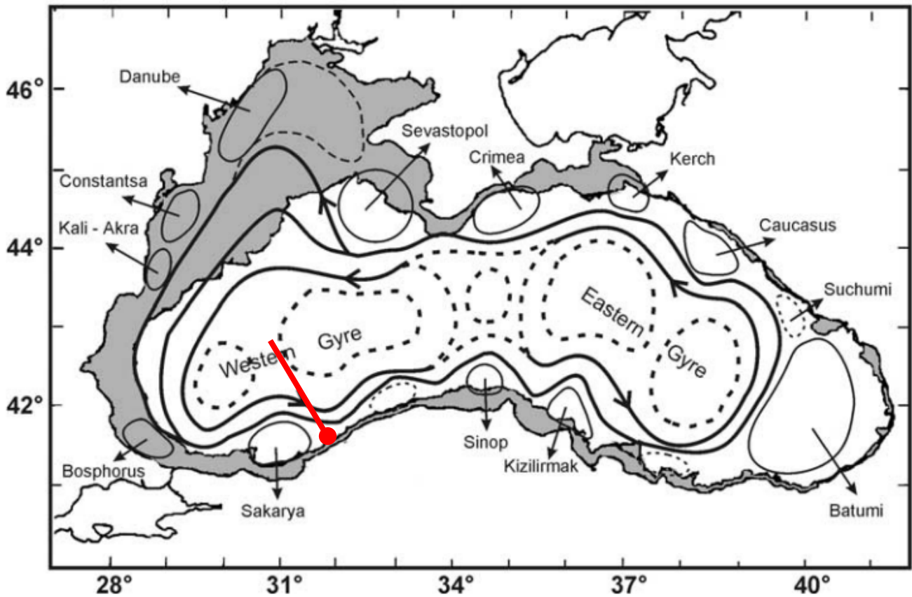
Figure 6-9: The Black Sea circulation (source: Korotaev et al., 2003). The red dot and line indicate the Project location.
