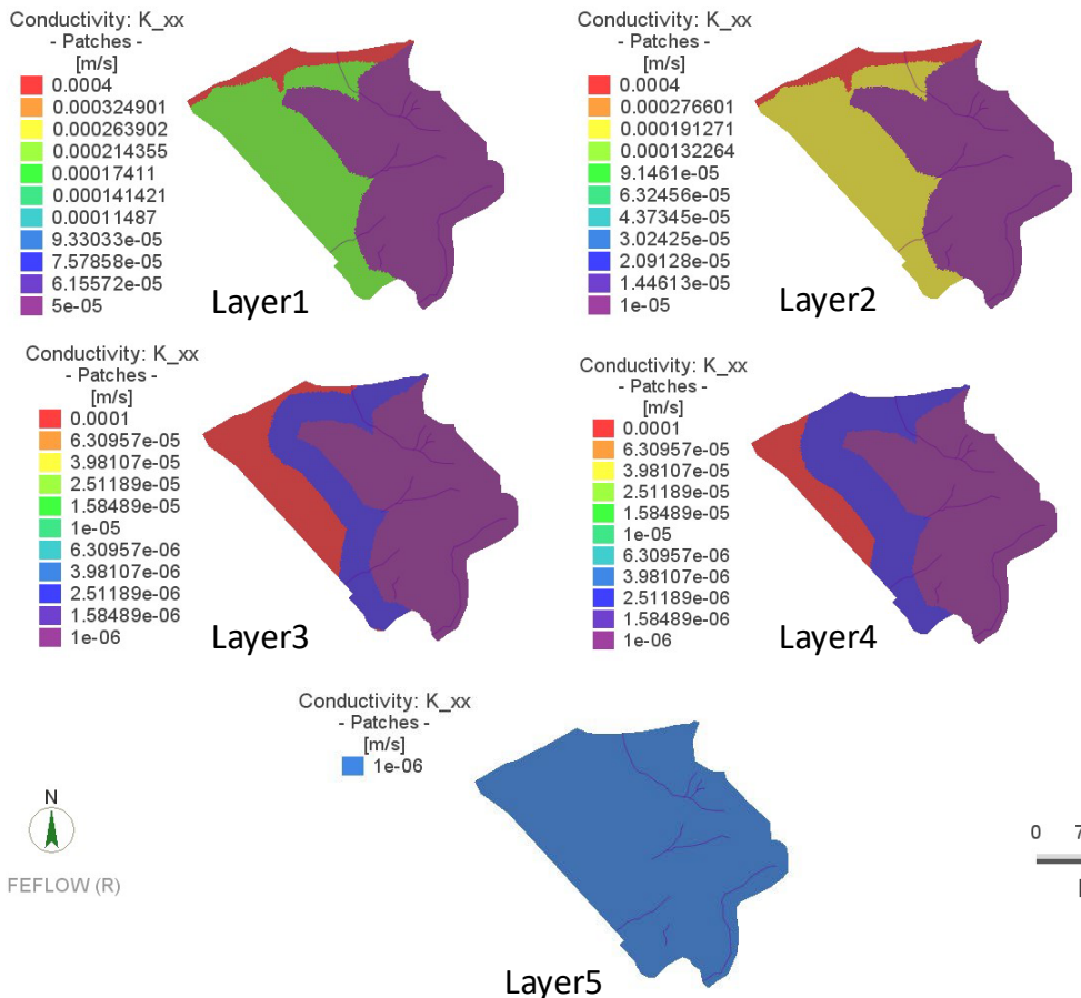
Figure 7-37: Hydraulic Conductivity (K) values assigned for each layer
