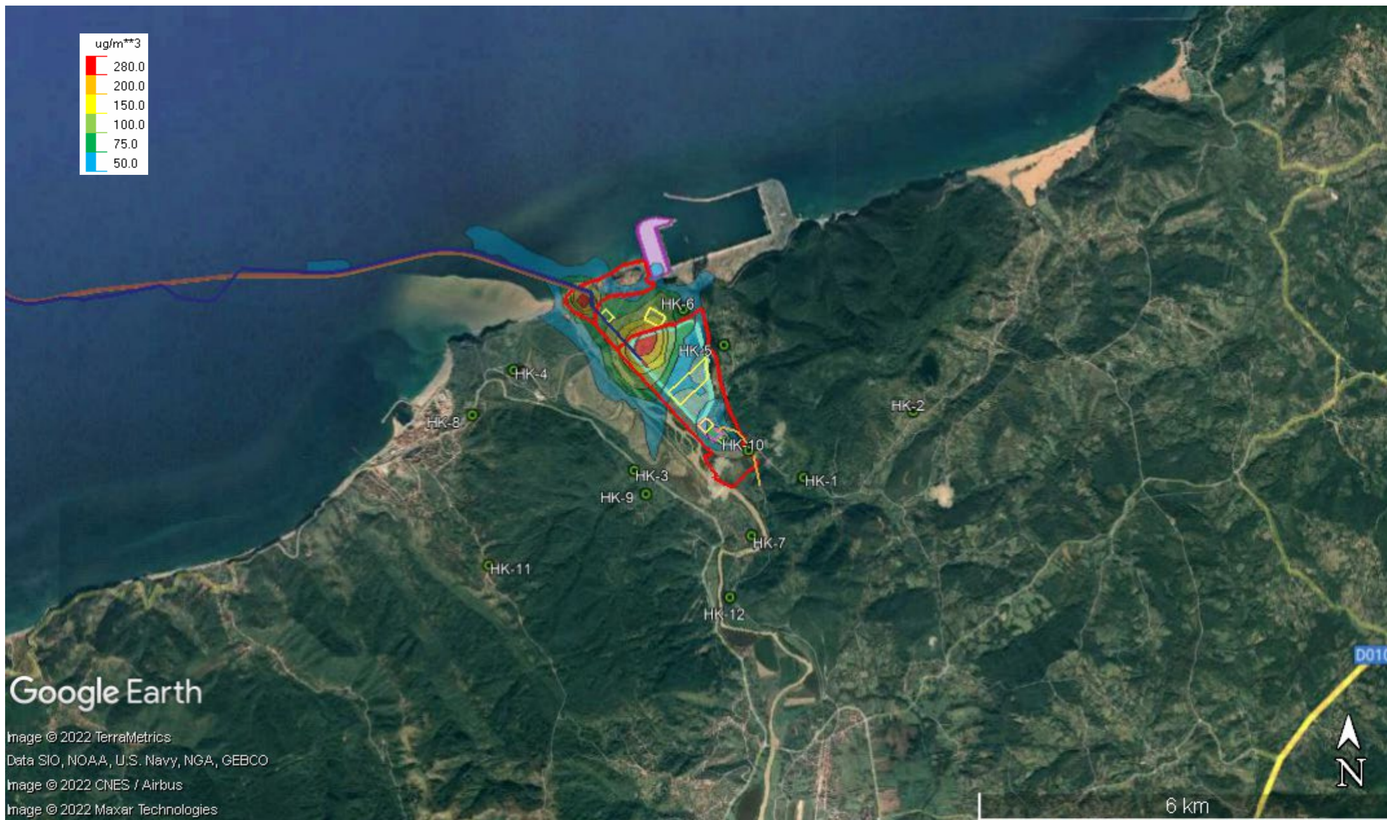
Figure 7-9: 1 st Highest 1-Hour Average GLC for VOC ( \mu\text{g}/\text{m}^3 )
