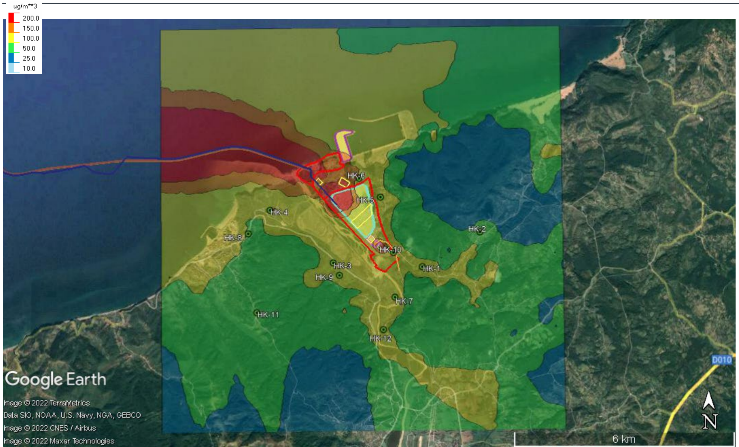
Figure 7-7: 6 th Highest 1-Hour Average GLC for NO 2 ( \mu\text{g}/\text{m}^3 )
