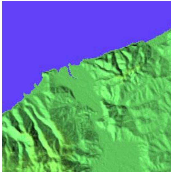
Figure 7-4: Terrain Elevations
