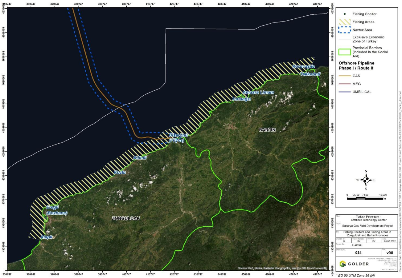
Figure 6-26: Fishing Areas
